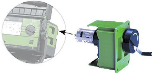
Hand Crank Generator
